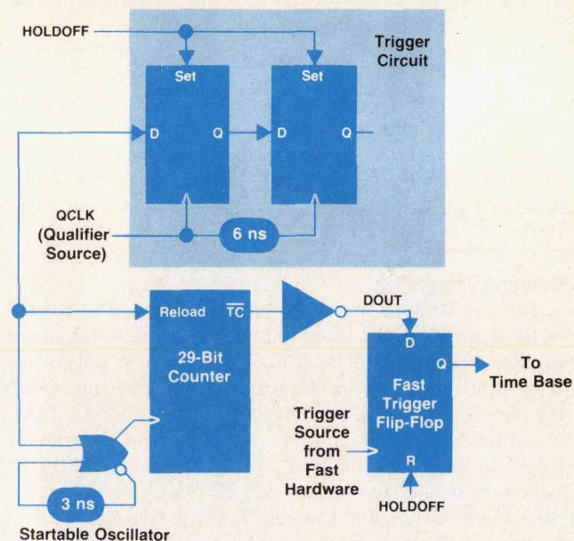
Fig. 8. Block diagram of the HP 54100AD triggering system in Time-Delay mode. The startable oscillator and counter are configured as a timer that is started by a trigger circuit. This allows time to be counted from an edge at QCLK before arming the fast trigger flip-flop.
