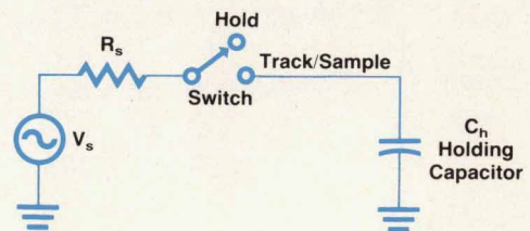
Fig. 8. Equivalent circuit of a track-and-hold or sample-and-hold circuit.
