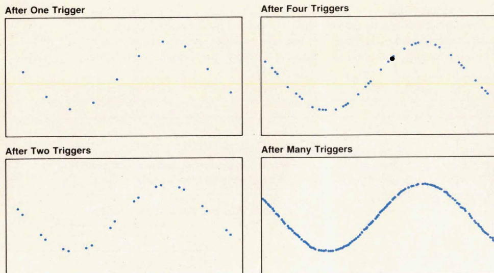
Fig. 1. In random repetitive sampling, the accumulation of information over many triggers or measurements produces an accurate image of the signal waveform.
