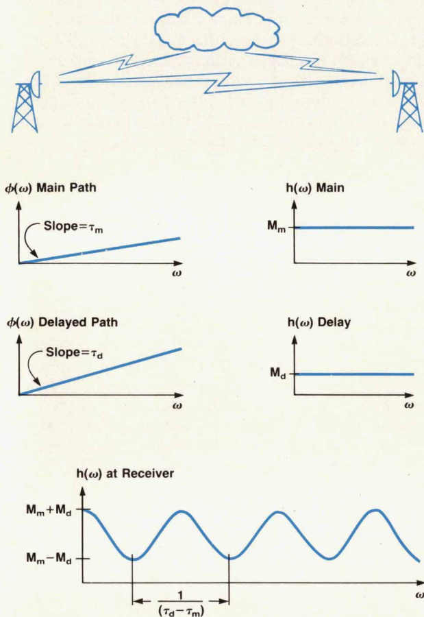
Fig. 7. The three most prevalent transmission paths for microwave signals are line-of-sight, diffractive, and reflective paths. The effect that multiple transmission paths have on the received digital microwave radio spectrum can be dramatic. Since a time delay results in a phase ramp in the frequency spectrum, the relative delay of one path with respect to another means that the phase of the delayed signal is shifted as a function of frequency with respect to the direct signal. When these add at the receiver, they add constructively or destructively depending on the specific frequency and delays. This results in a sinusoidal ripple in the received frequency spectrum, which when plotted on a log scale, appears as notches. The depth of the notches is a function of the amplitudes of the main and delayed signals, and their separation in the frequency domain is inversely proportional to the differential delay. By modeling the multipath fade with a frequency dependent phase shift, I•Q Tutor accurately simulates many of the effects of a real multipath fade.
