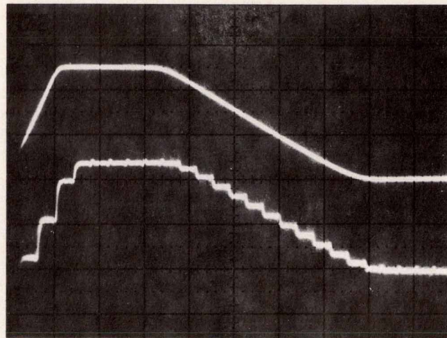
Fig. 13. A ramp-type input to the sampler and the output of the postamplifier held in steps 25 ns apart.
