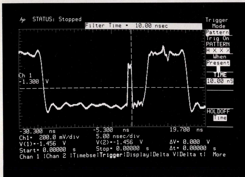
Fig. 7. Trace of a 1-ns glitch occurring within a complex data stream. The trigger is solidly locked onto the 1-ns glitch while rejecting pulses of longer duration, including the one that occurs only 5 ns later.
