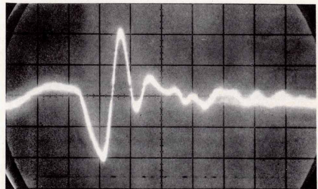
Fig. 5. Sampler kickout. Vertical: 5 mV/div. Horizontal: 200 ps/div.
